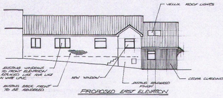
PROPOSED EAST ELEVATION
