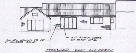
PROPOSED WEST ELEVATION
